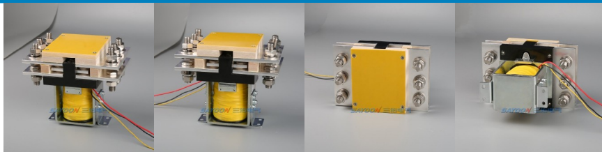
Product name: Magnetic Holding DC Contactor Product type: CZWH1600A-K Rated load current: 1600A Contact form: 2 Circuit
