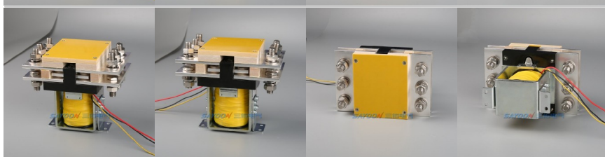
Product name: Magnetic Holding DC Contactor Product type: CZWH3000A-K Rated load current: 3000A Contact form: 2 Circuit
